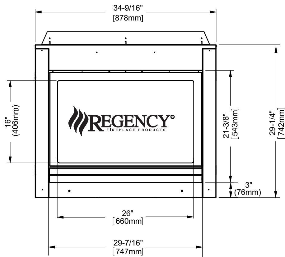
FRONT VIEW
